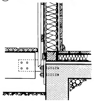
14 Replaceable beams or terrace supports
